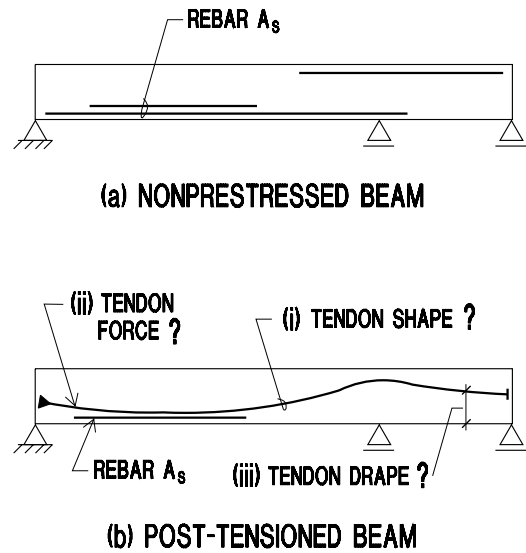
Fig.1: Schematic comparing a conventionally reinforced concrete member to a post-tensioned member. Notice the assumptions required for the post-tensioned design
