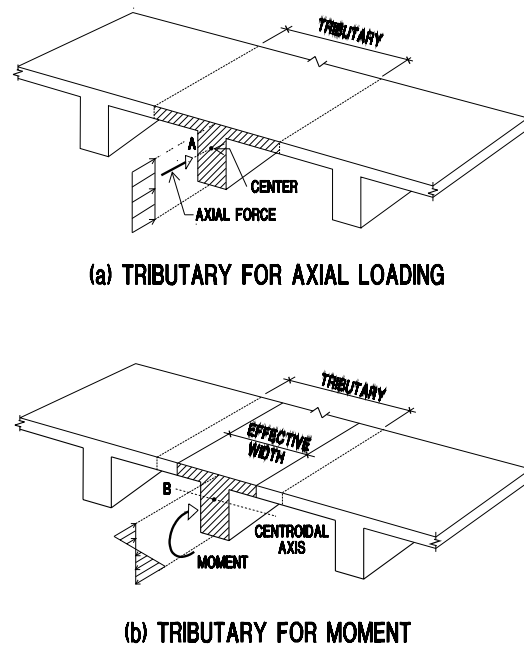
Fig.2: Tributaries used when computing average precompression stress for stemmed members.
