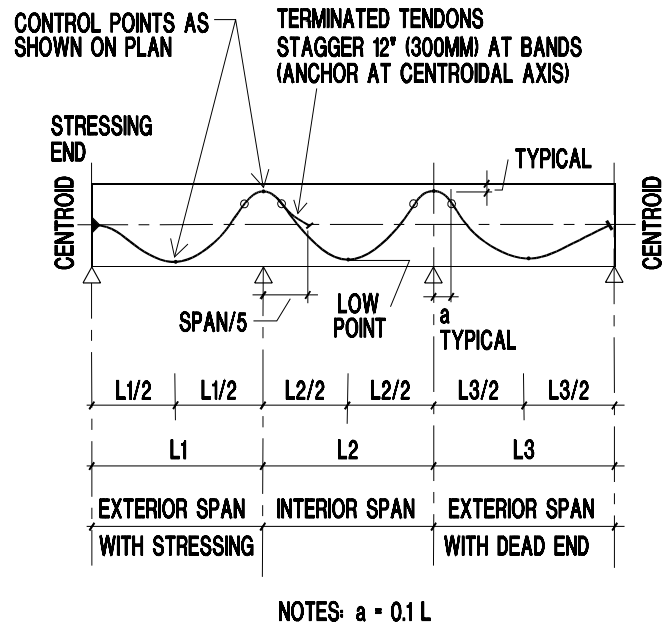
Fig.5: For tendons in the distributed direction of beams and slabs, the tendon profile is a reversed parabola with inflection points at one-tenth the span length
